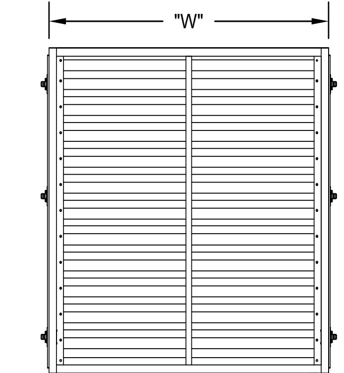
1 5/16" FLANGE WIDTH, ALL SIDES FLANGE CONNECTION
