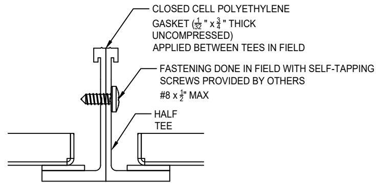
A HALF TEE FIELD JOINT
