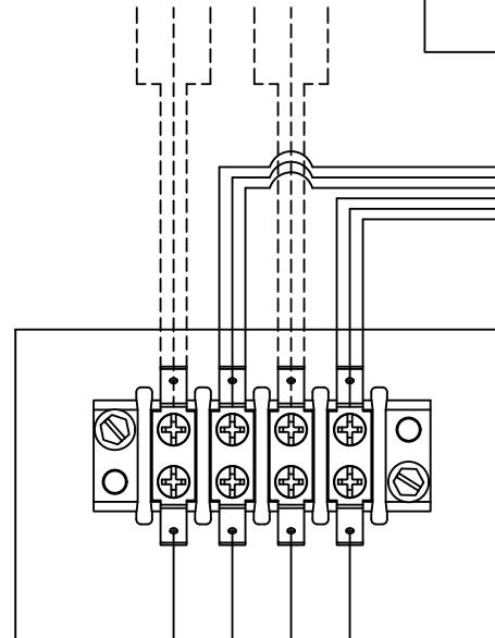
600W DRIVER NEGATIVE LOW VOLTAGE FIELD CONNECTIONS
