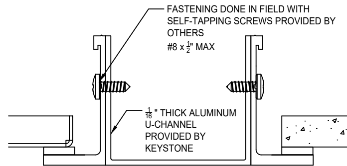
C U CHANNEL DETAIL
