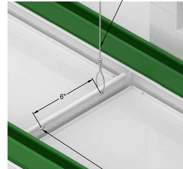
TYPICAL HANGER WIRE LOCATION
