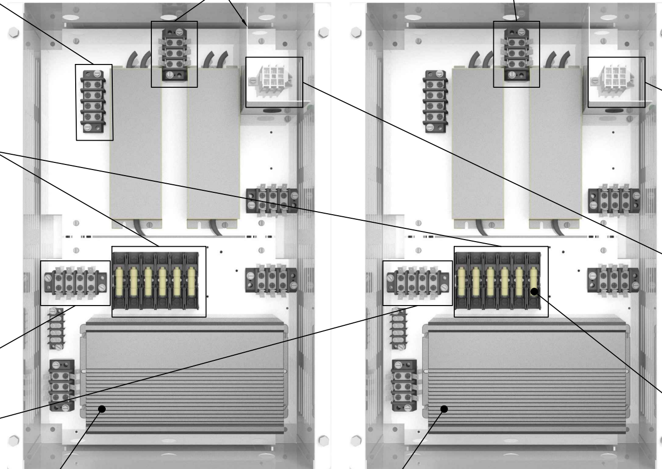
SRDC-2-X REMOTE DRIVER CABINET TYPE CD SHOWN
