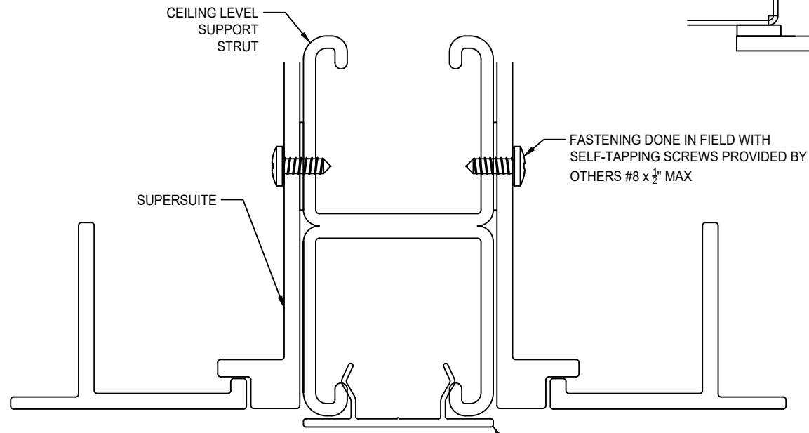
D SSA UNISTRUT INTEGRATION
