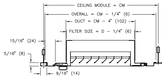
Border 17 - 9/16" Tegalor or Bolt Slot Tee
