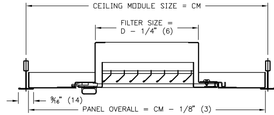
Border 916P/916PA – For 9/16" Flat Tee
