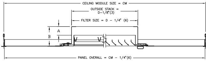
Border 3P/3PA – For 15/16" Flat Tee
