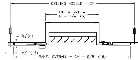
Border 17P/17PA – For 9/16" Tegular or Bolt Slot Tee
