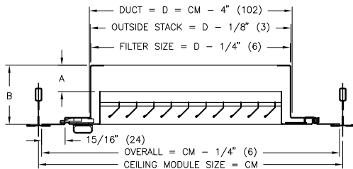
Border TB – 15/16" Flat Tee
